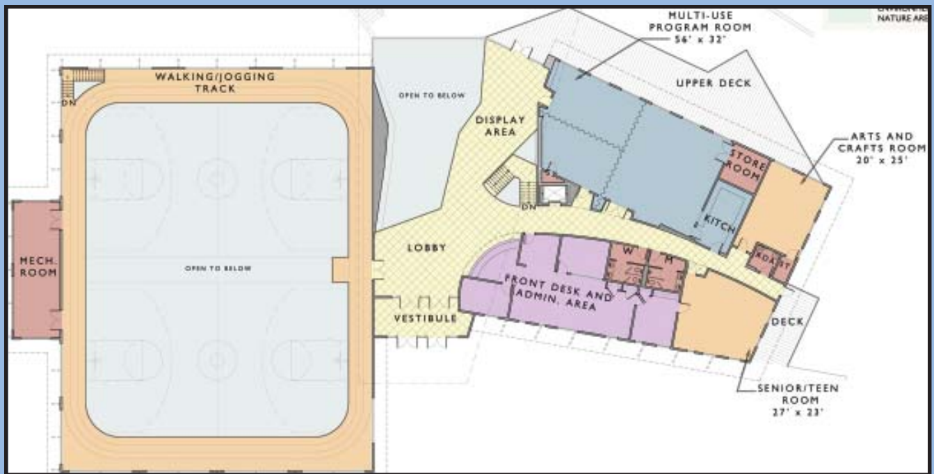
Upper Level Floor Plan
